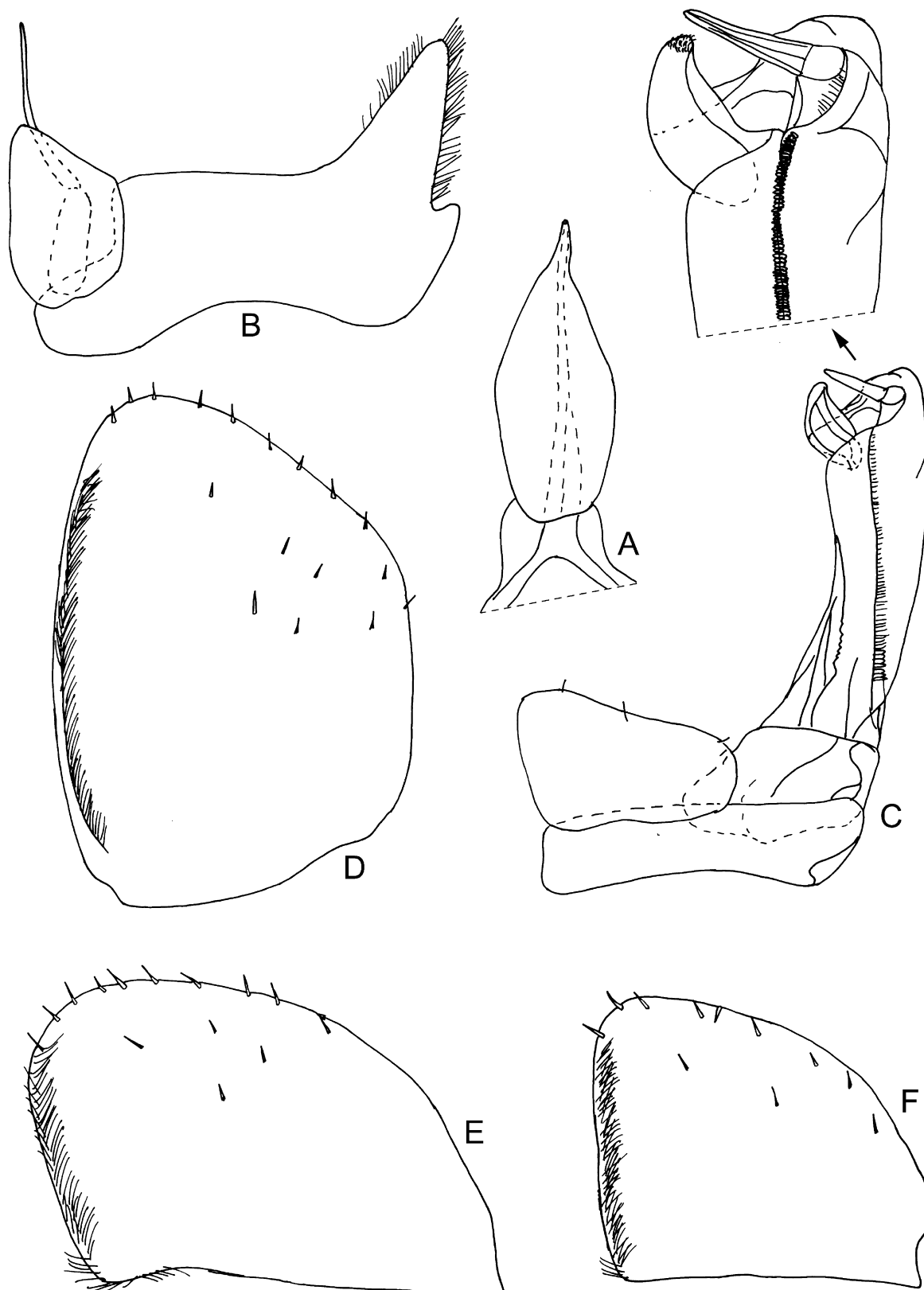
Figure 13. Xangoniscus aganju Campos-Filho, Araujo & Taiti sp. nov. , ♂: A, genital papilla; B, pleopod 1; C, pleopod 2; D, pleopod 3 exopod; E, pleopod 4 exopod; F, pleopod 5 exopod.
